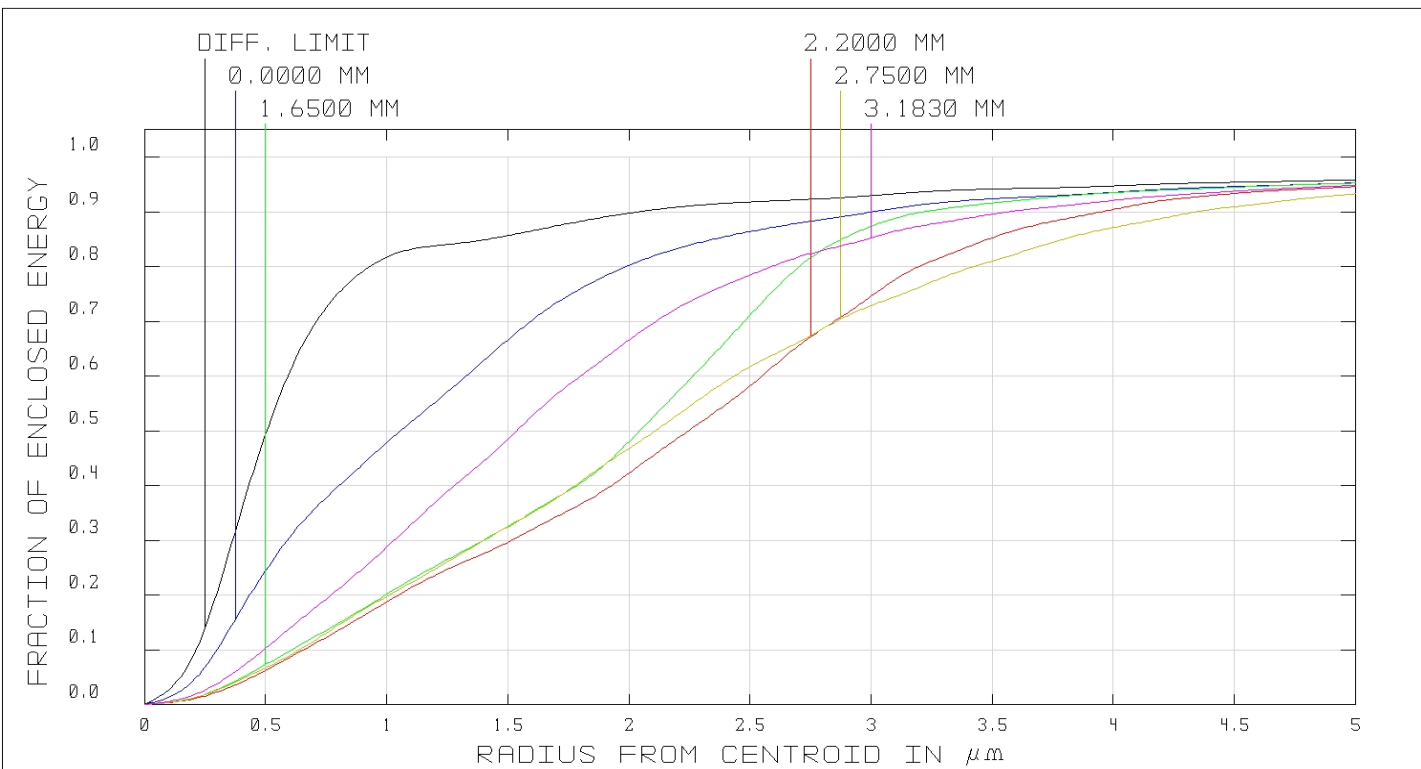
FFT DIFFRACTION ENCIRCLED ENERGY
